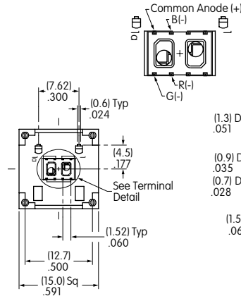
Terminal Detail
