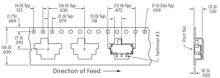
Tape Dimensions
