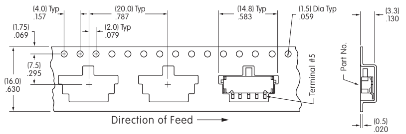
Tape Dimensions
