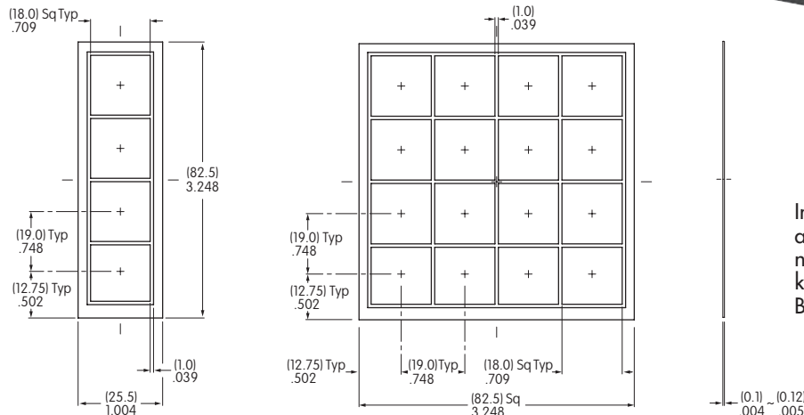
Insertable Legend Card for 4 Key or 16 Key
