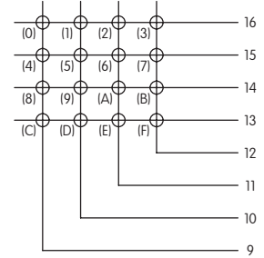
LED Circuit Matrix For 16 Key
