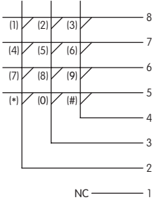
Switch Circuit Matrix For 12 Key
